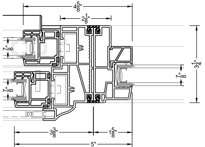
④ 0 DEGREE MULLION DH200 & PW211
