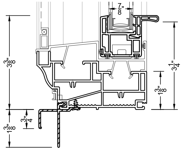
②A SILL - APPLIED J-CHANNEL DH200
