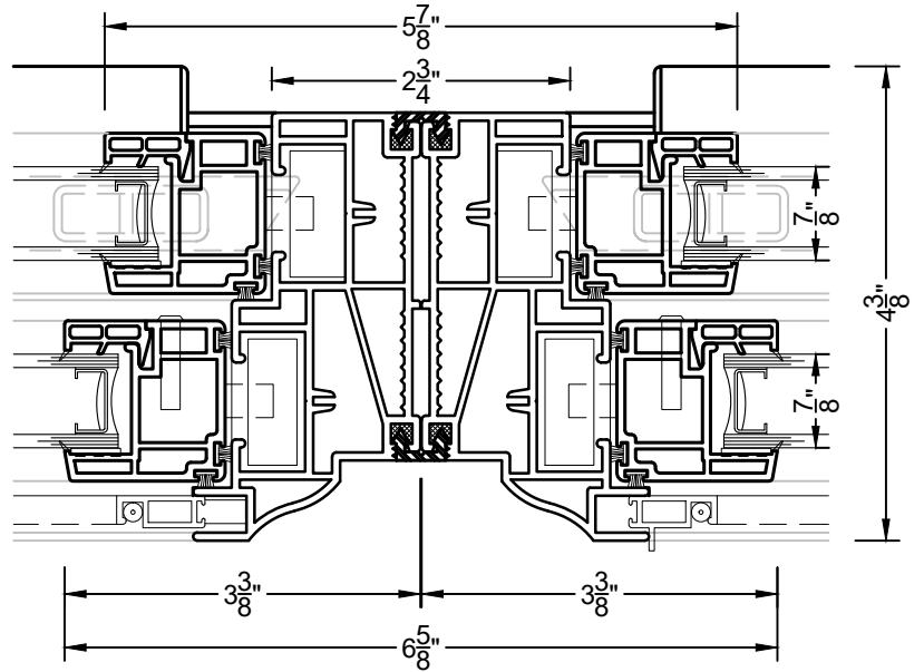
③ 0 DEGREE MULLION DH200 & DH200
