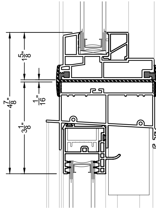
① H-MULLION PW211 OVER DH100
