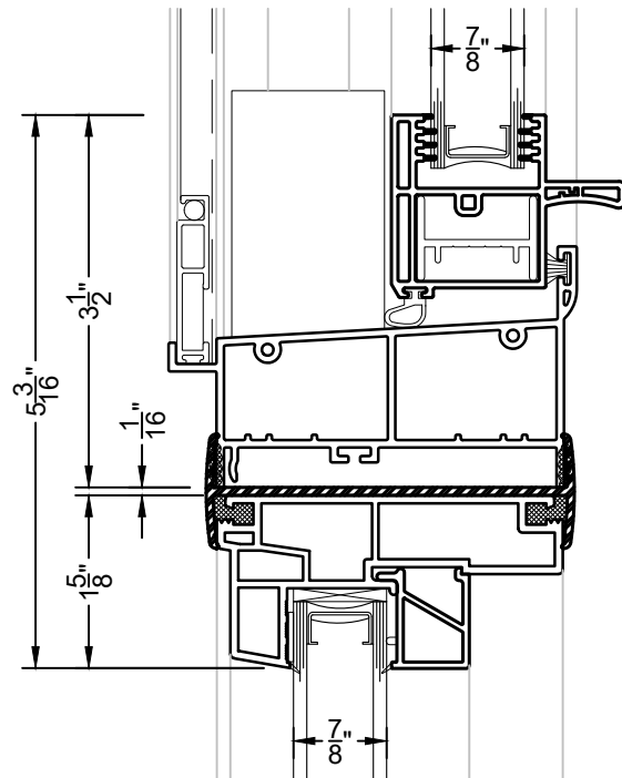
② H-MULLION DH100 OVER PW211
