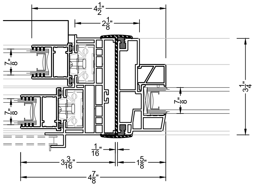
② H-MULLION DH100 & PW211
