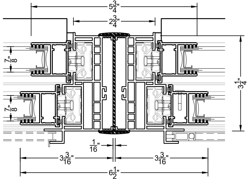
① H-MULLION DH100 & DH100
