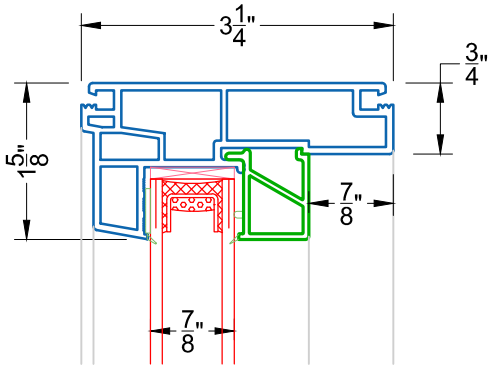
1 STANDARD HEAD PW 211
