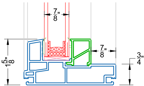
2 STANDARD SILL PW 211
