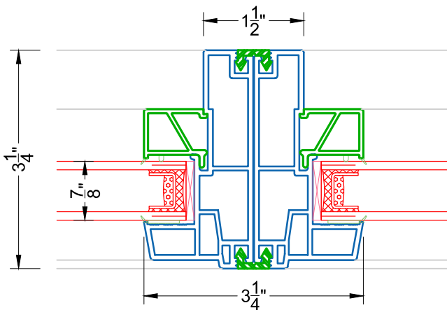
5 0 DEGREE MULLION PW 211
